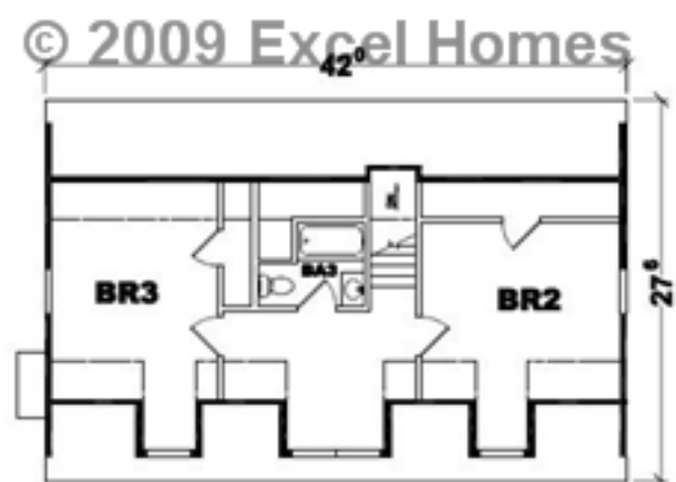
Proposed Second Floor Layout
